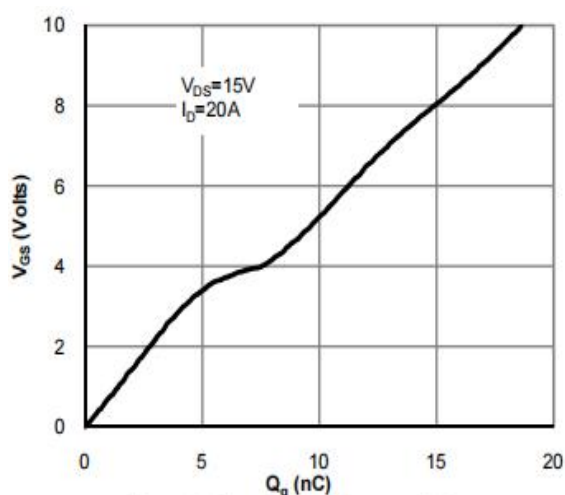
Figure 6: Gate-Charge Characteristics
