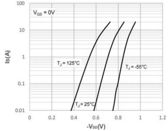
Figure 2: Diode Characteristics
