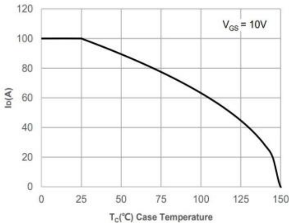
Figure 9: Current De-rating
