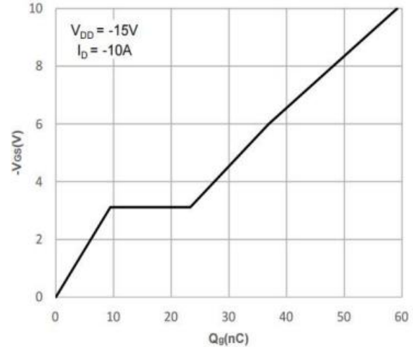
Figure 6: Gate-Charge Characteristics
