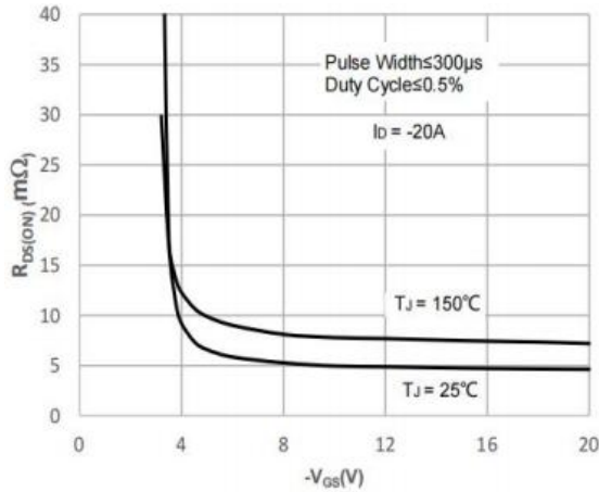
Figure 3: On-Resistance vs. V_{GS}
