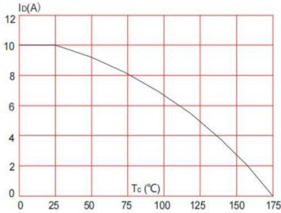
Figure 7: Drain Current Characteristics
