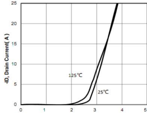
-V GS Gate-Source Voltage (V)
