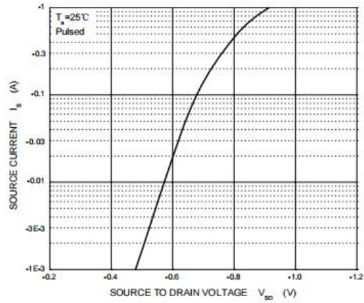
Figure 4: Diode Characteristics
