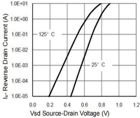
Figure 7: Diode Characteristics
