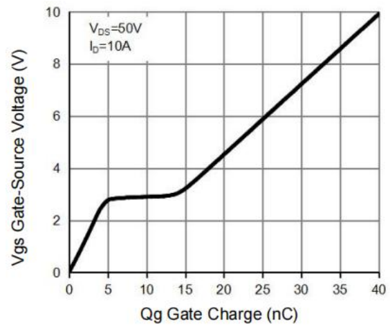
Figure 6: Gate-Charge Characteristics
