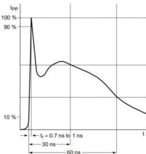
IEC61000-4-2 Waveform
