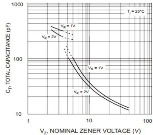
Figure 4: Capacitance Characteristics
