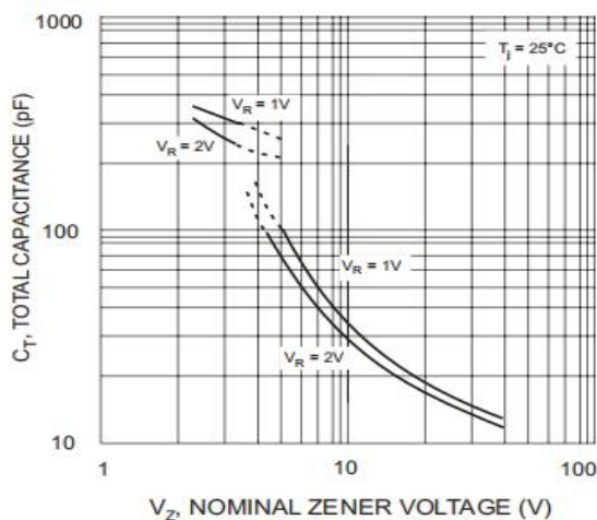
Figure 2: Capacitance Characteristics
