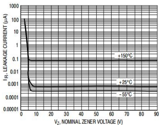
Figure 5: Leakage Current
