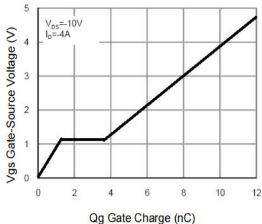
Figure 6: Gate-Charge Characteristics
