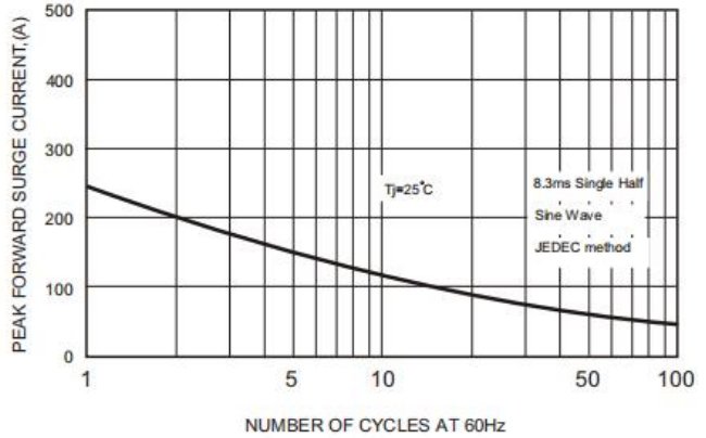
Figure 2: Peak Forward Surge Current
