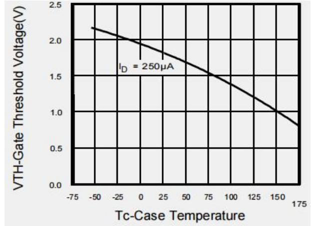
Figure 8: Threshold Voltage vs. T C
