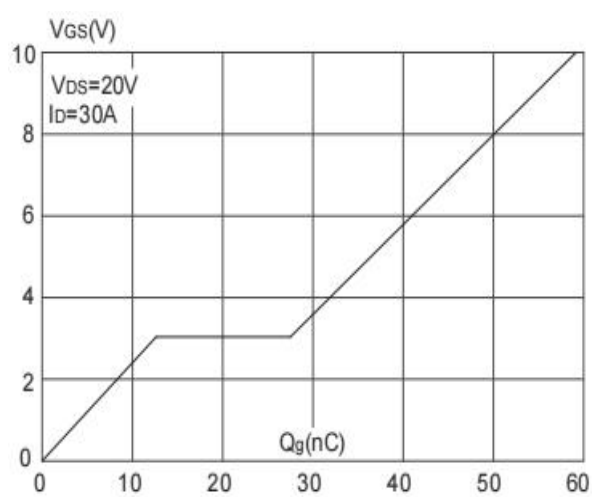
Figure 6: Gate-Charge Characteristics
