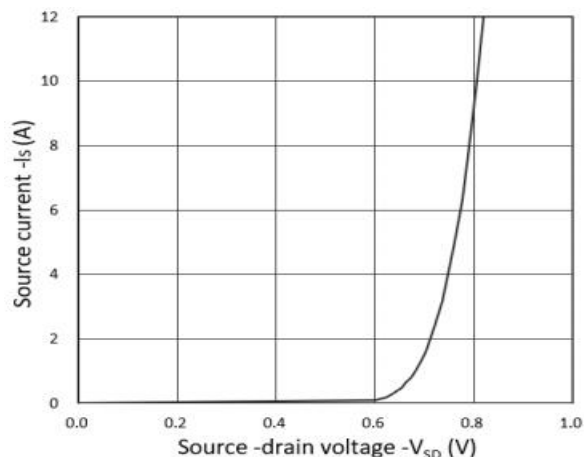
Figure 2: Diode Characteristics
