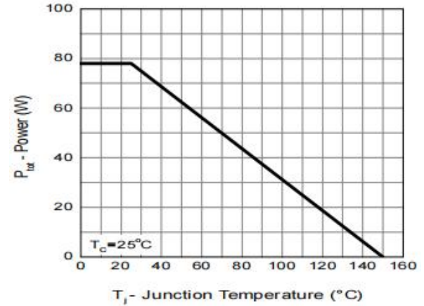
Figure 8: Power Rating Characteristics
