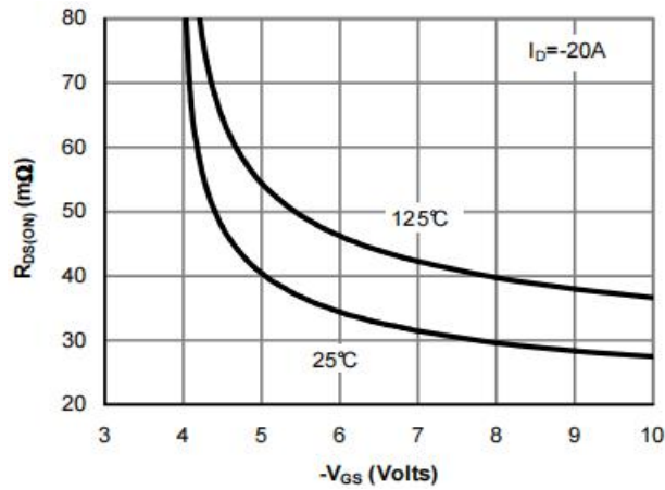
Figure 9: On-Resistance vs. Threshold Voltage
