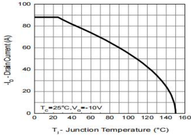
Figure 9: Drain Current Characteristics
