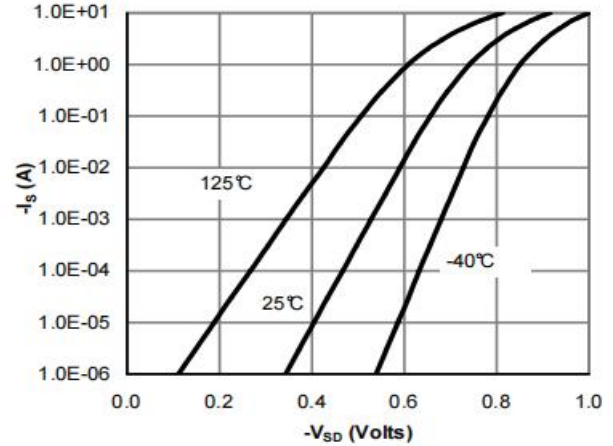
Figure 2: Diode Characteristics
