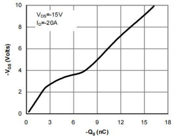
Figure 6: Gate-Charge Characteristics
