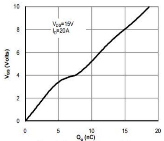
Figure 6: Gate-Charge Characteristics
