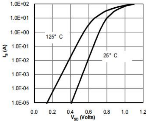
Figure 9: Diode Characteristics
