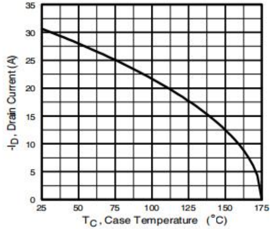
Figure 8: Drain Current Characteristics
