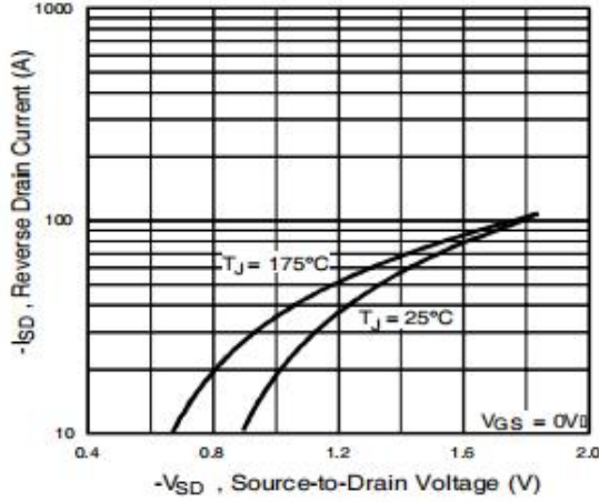
Figure 7: Diode Characteristics
