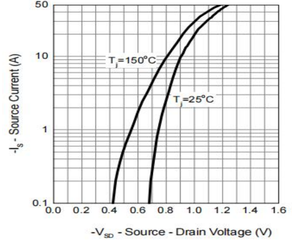
Figure 2: Diode Characteristics
