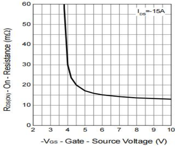
Figure 9: On-Resistance vs. Threshold Voltage
