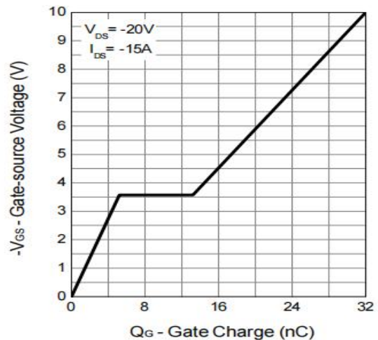
Figure 6: Gate-Charge Characteristics
