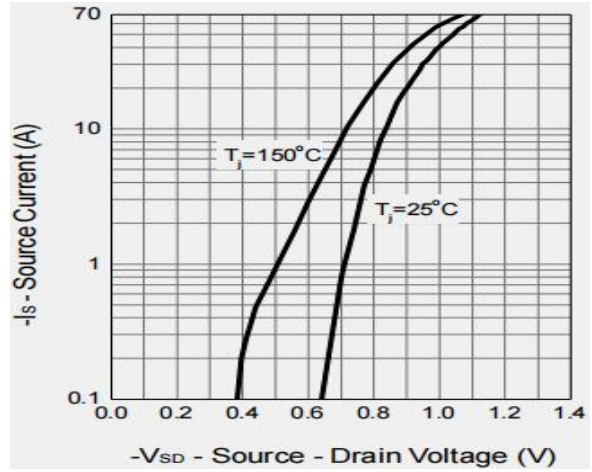
Figure 2: Diode Characteristics
