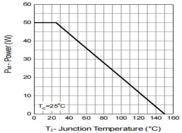
Figure 4: Power Rating Characteristics
