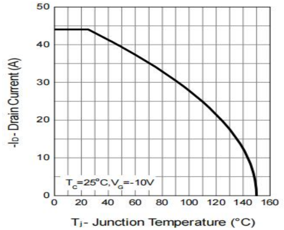
Figure 8: Drain Current Characteristics
