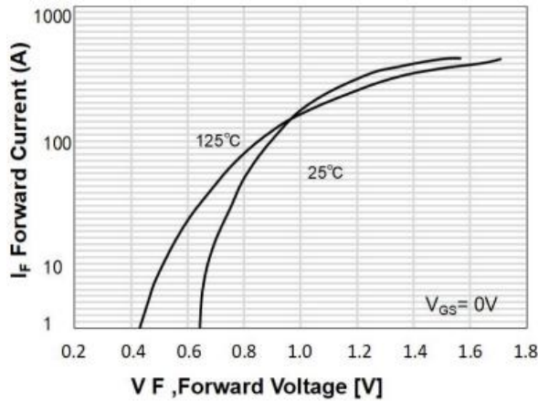
Figure 9: Diode Characteristics
