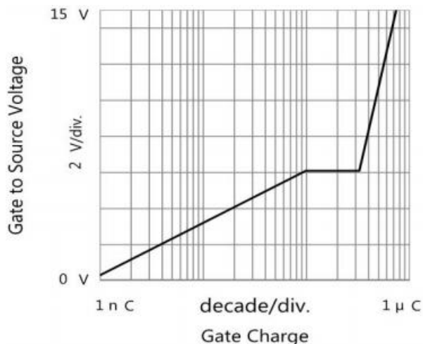
Figure 6: Gate-Charge Characteristics
