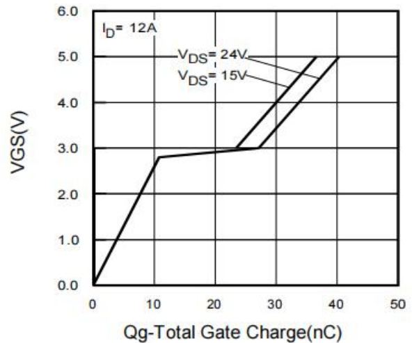
Figure 6: Gate-Charge Characteristics
