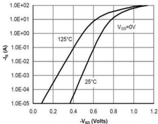
Figure 8: Diode Characteristics
