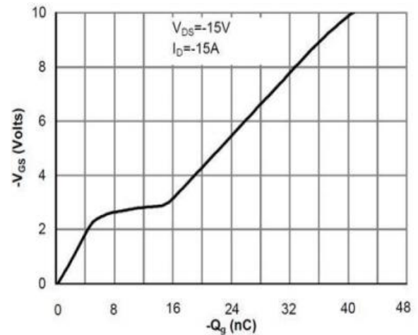
Figure 6: Gate-Charge Characteristics
