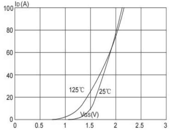
Figure 4: Transfer Characteristics
