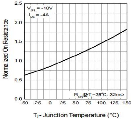
Figure 3: On-Resistance vs. T_J
