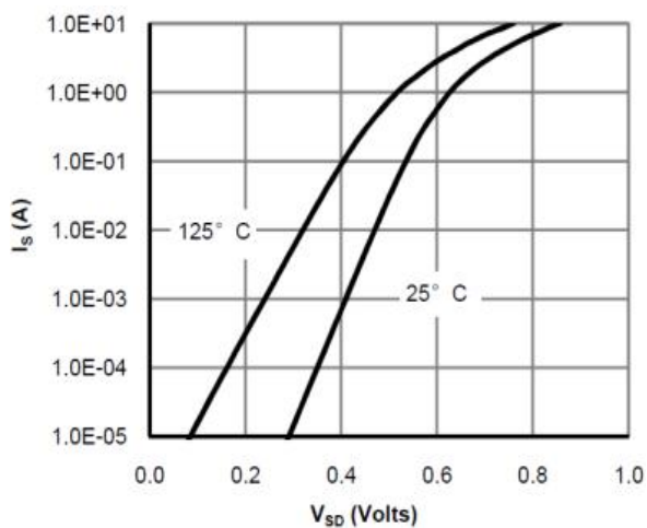
Figure 9: Diode Characteristics
