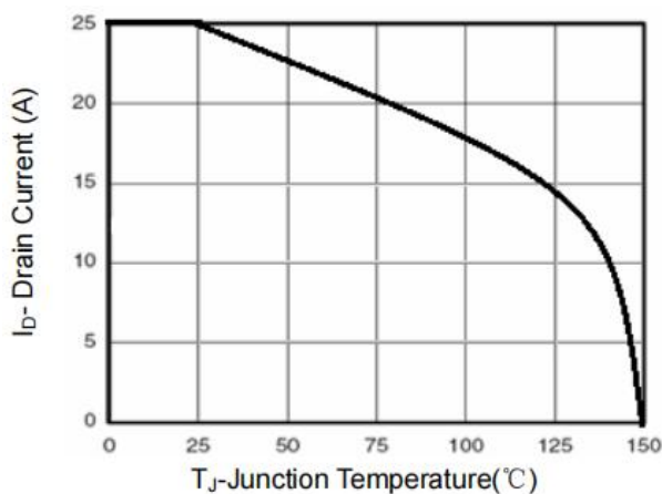
Figure 9: Current Rating Curve
