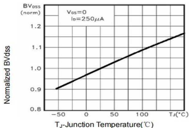
Figure 8: Breakdown Voltage vs. T_J
