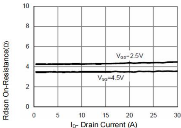
Figure 7: On-Resistance vs. Drain Current
