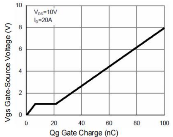
Figure 6: Gate-Charge Characteristics
