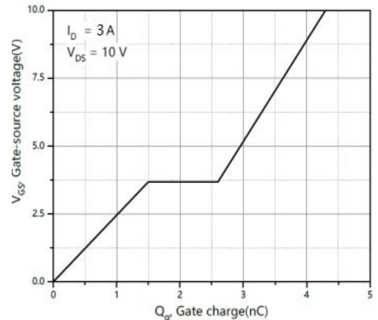
Figure 6: Gate-Charge Characteristics
