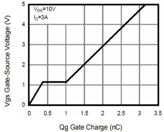
Figure 6: Gate-Charge Characteristics
