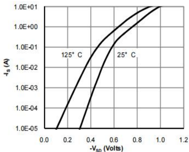
Figure 8: Diode Characteristics
