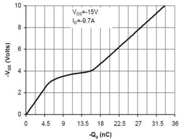
Figure 6: Gate-Charge Characteristics
