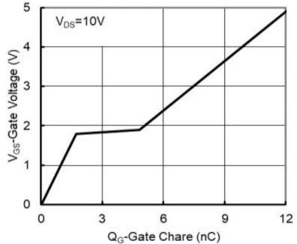
Figure 6: Gate-Charge Characteristics
