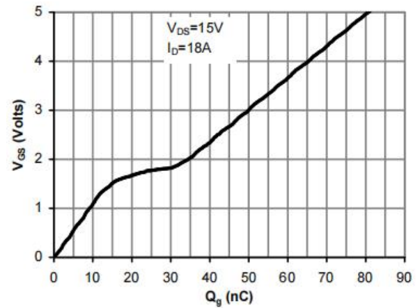
Figure 6: Gate-Charge Characteristics
