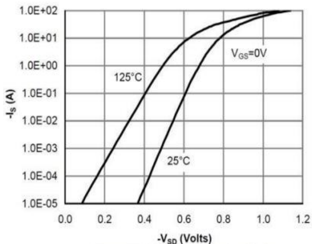
Figure 8: Diode Characteristics
