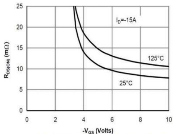
Figure 10: On-Resistance vs. Vgs
