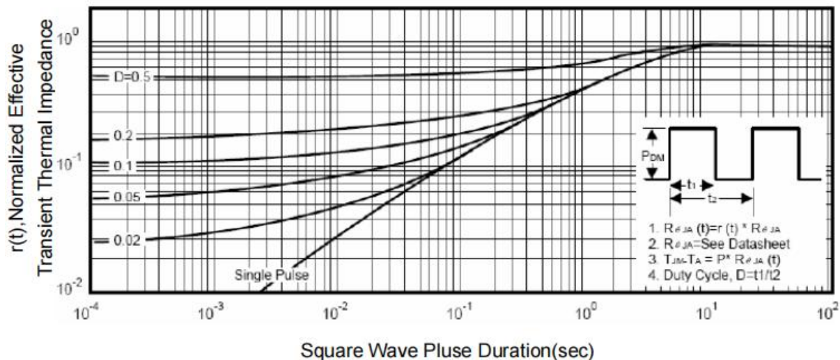
Figure 9: Transient Thermal Response Curve
