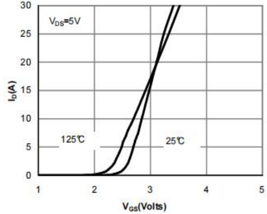
Figure 4: Transfer Characteristics
