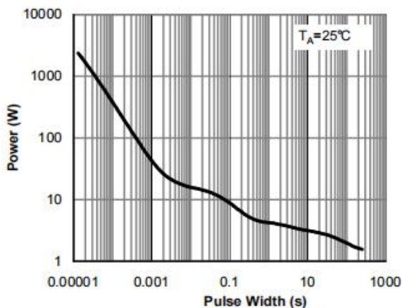
Figure 9: Power Rating Curve
