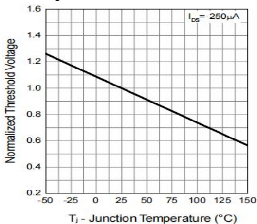
Figure 4: Gate Threshold Voltage
