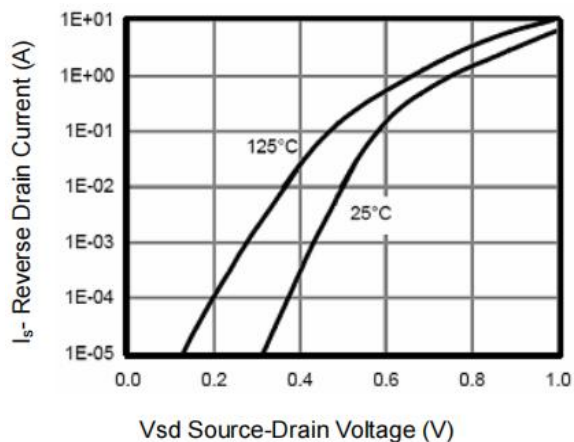
Figure 9: Diode Characteristics
