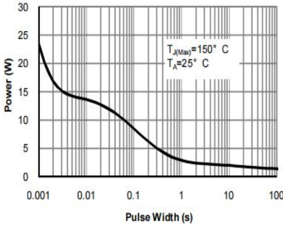
Figure 9: Power Rating Curve
