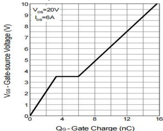
Figure 6: Gate-Charge Characteristics
