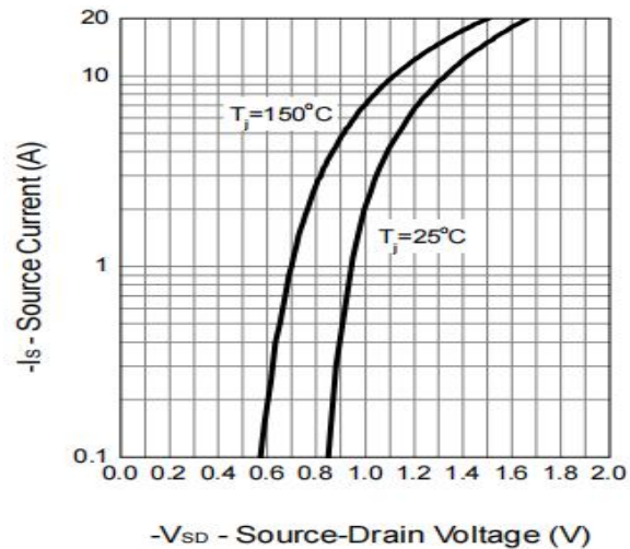
Figure 2: Diode Forward Characteristics
