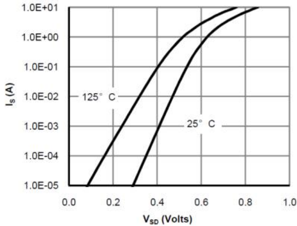
Figure 9: Diode Characteristics
