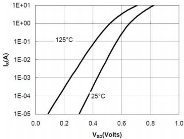
Figure 9: Diode Characteristics
