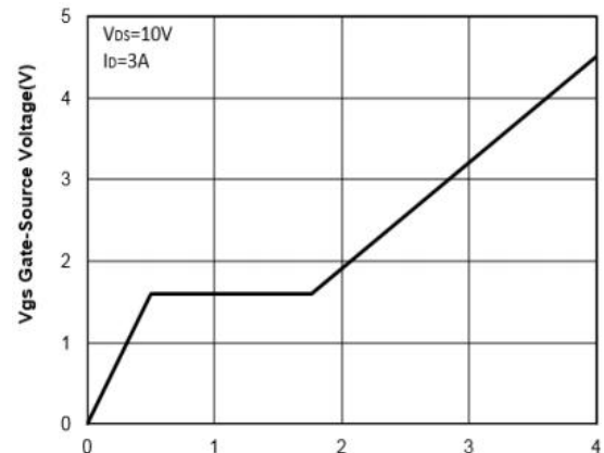
Qg Gate-Charge (nC) Figure 6: Gate-Charge Characteristics
