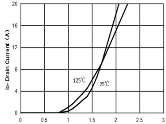
V GS Gate-Source Voltage (V) Figure 2: Transfer Characteristics
