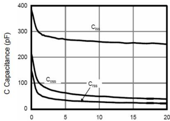
V DS Drain-Source Voltage (V) Figure 5: Capacitance Characteristics
