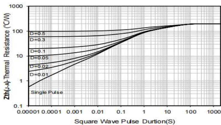
Figure 9: Transient Thermal Response Curve
