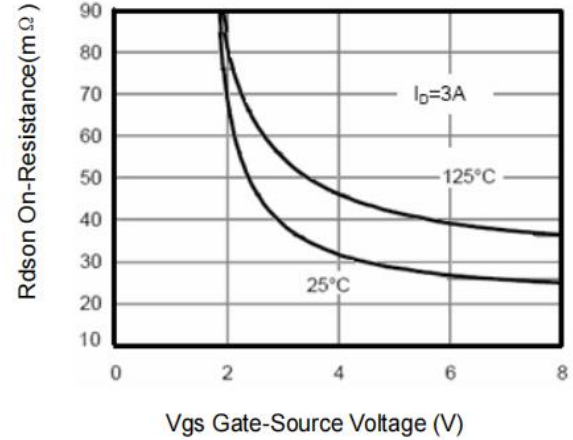
Figure 8: On-Resistance vs. V_{GS}
