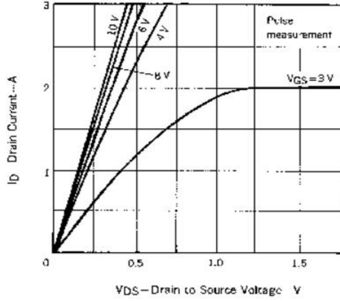
Figure 1: Output Characteristics
