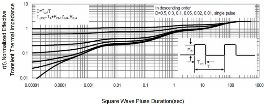
Figure 10: Transient Thermal Response Curve
