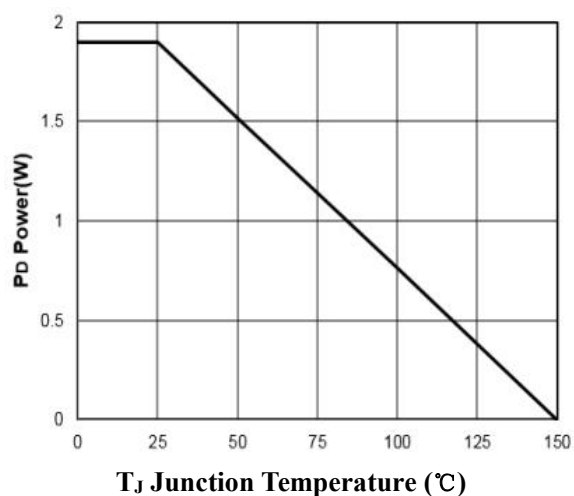
Figure 8: Power Dissipation
