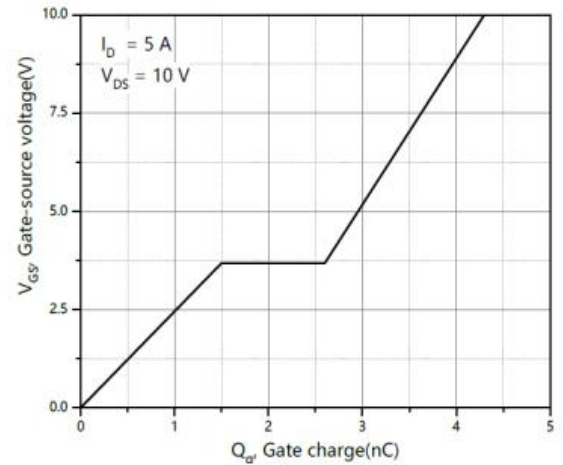
Figure 6: Gate-Charge Characteristics
