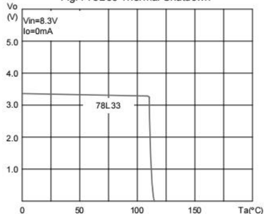
Fig.4 78L33 Thermal Shutdown
