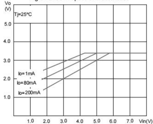
Fig.6 78L33 Dropout Characteristics
