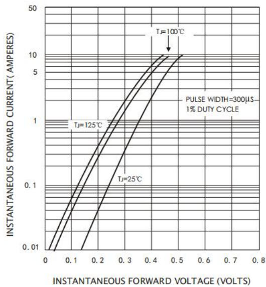
Figure 3: Forward Characteristics
